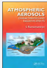
Atmospheric Aerosols: Characteristics and Radiative Effects
